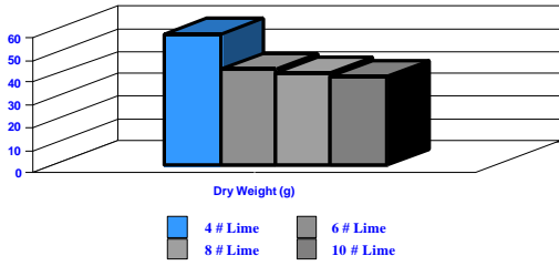
Figure 1. Hinodegiri Azalea Top Growth
