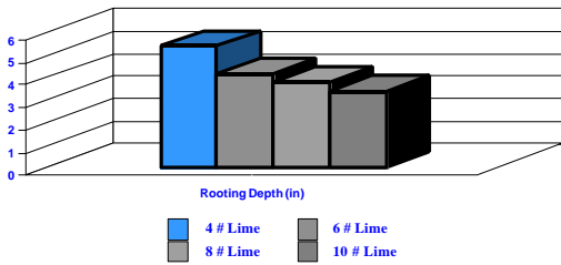
Figure 2. Hinodegiri Azalea Root Growth
